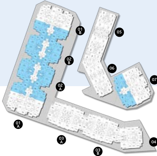
Typical floor plan of buildings 01-B, 02-B, 01-A, 02-A and 07
